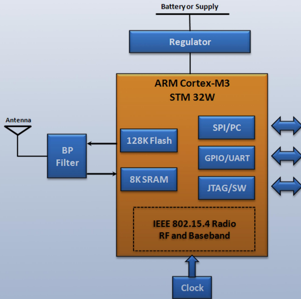
ZB 23 ZigBee Module Block Diagram
